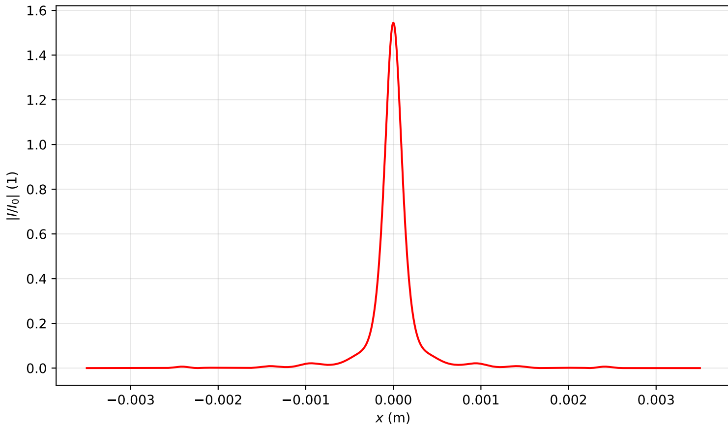
Intensity profile I(x, y = 0, z = 3.184)/I_0 , P_{in}=4.0P_{cr} , artificial time
